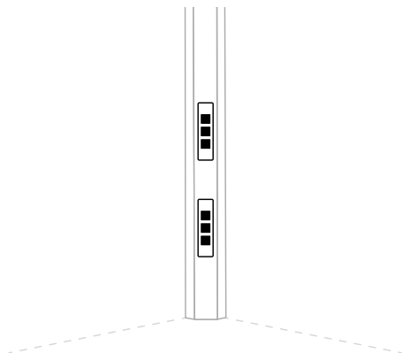
Power Modules
